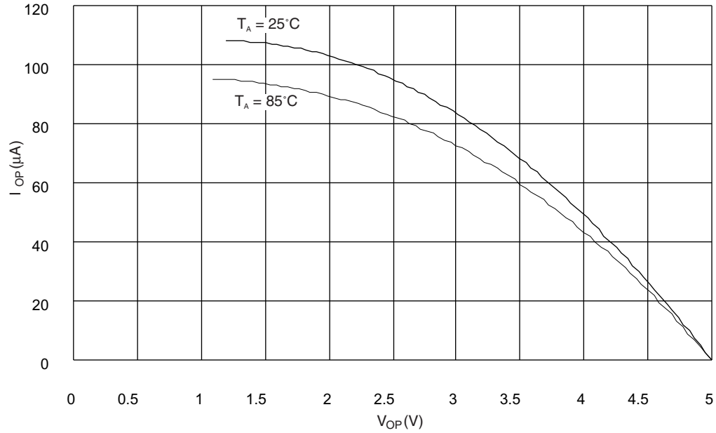
Figure 47. Pull-up Resistor Current vs. Input Voltage ( V_{CC}=2.7V )
