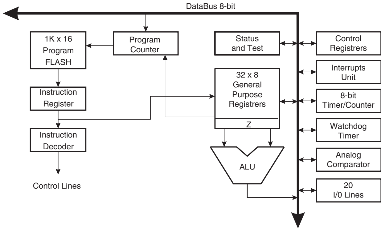
Figure 5. The ATtiny28 AVR RISC Architecture
