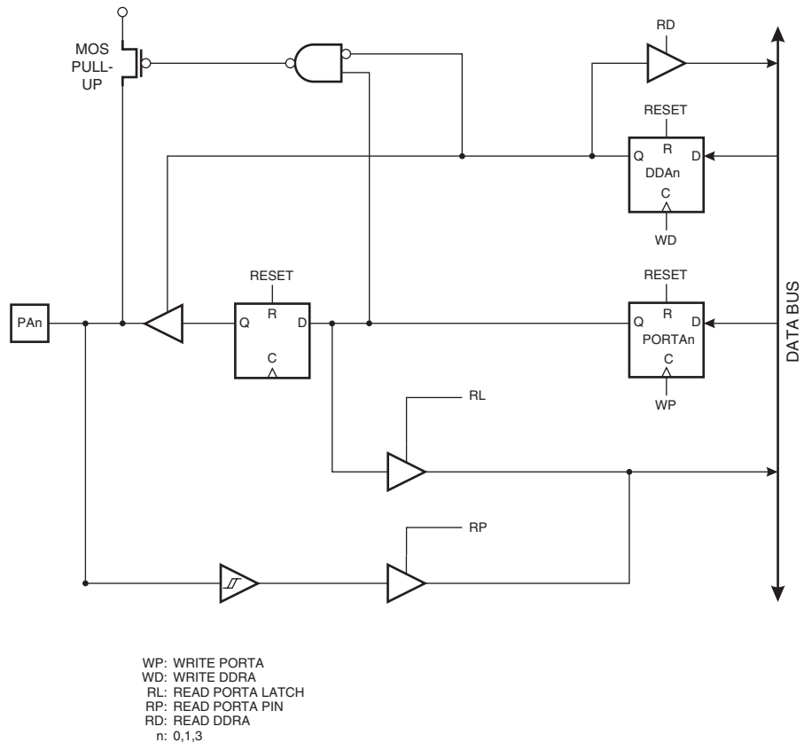
Figure 29. Port A Schematic Diagram (Pins PA0, PA1 and PA3)
