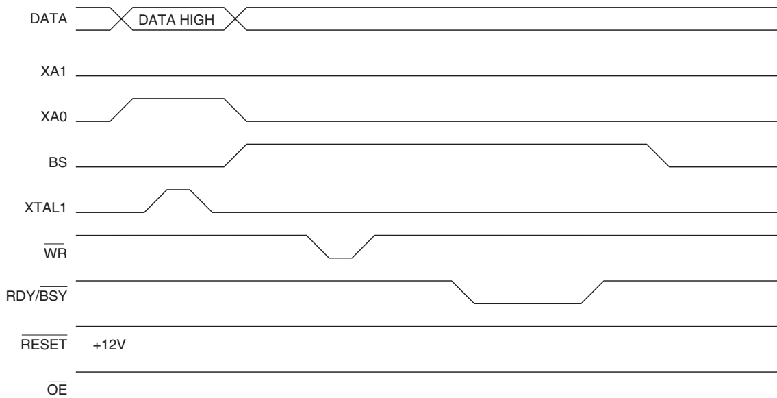
Figure 38. Programming the Flash Waveforms (continued)
