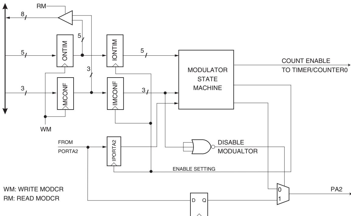
Figure 23. The Hardware Modulator
