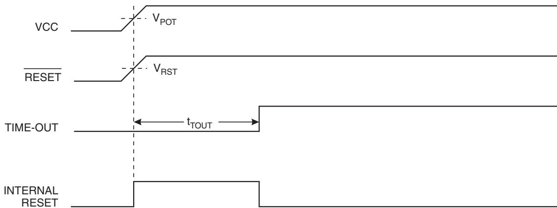
Figure 16. MCU Start-up, \overline{\text{RESET}} Tied to V_{CC} .
