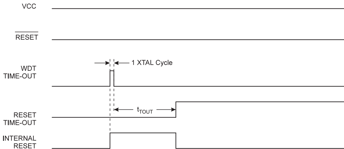
Figure 19. Watchdog Reset During Operation
