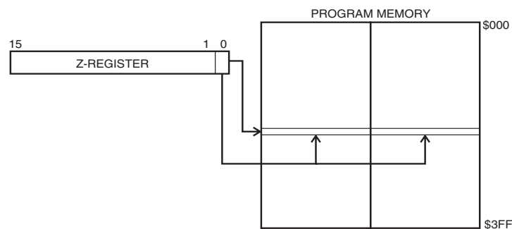
Figure 12. Code Memory Constant Addressing
