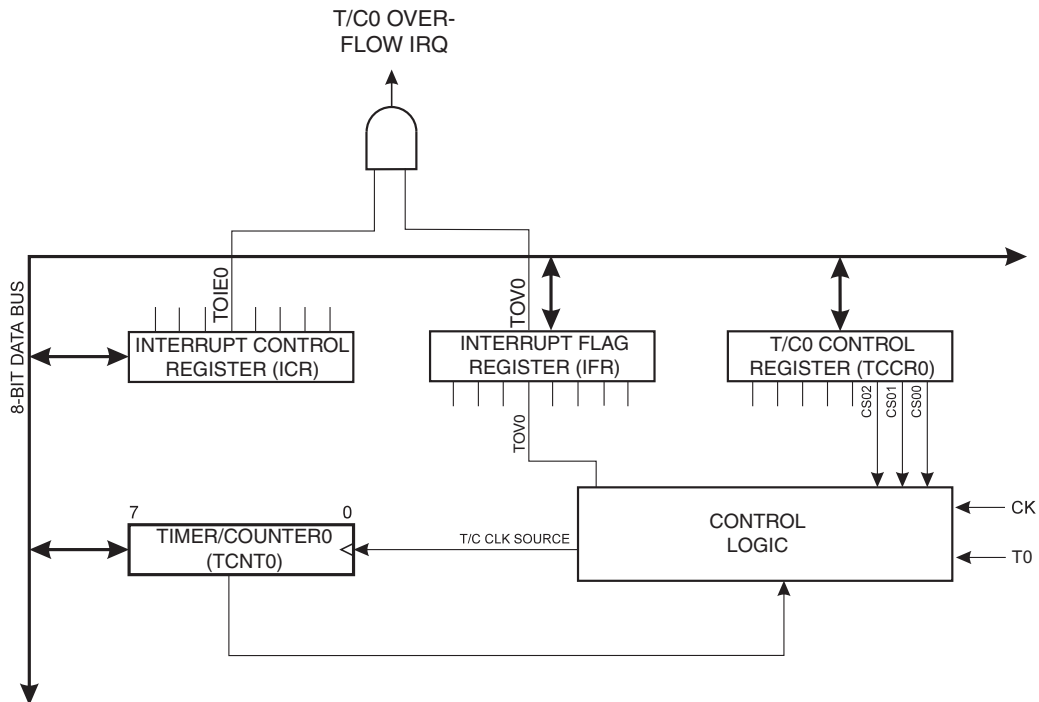
Figure 21. Timer/Counter0 Block Diagram
