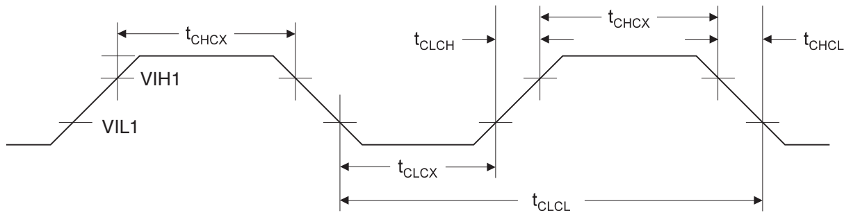
Figure 40. External Clock
