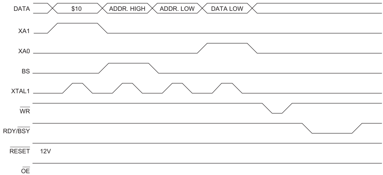
Figure 37. Programming the Flash Waveforms
