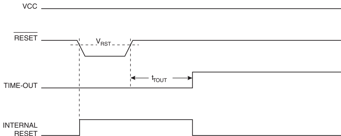
Figure 18. External Reset During Operation
