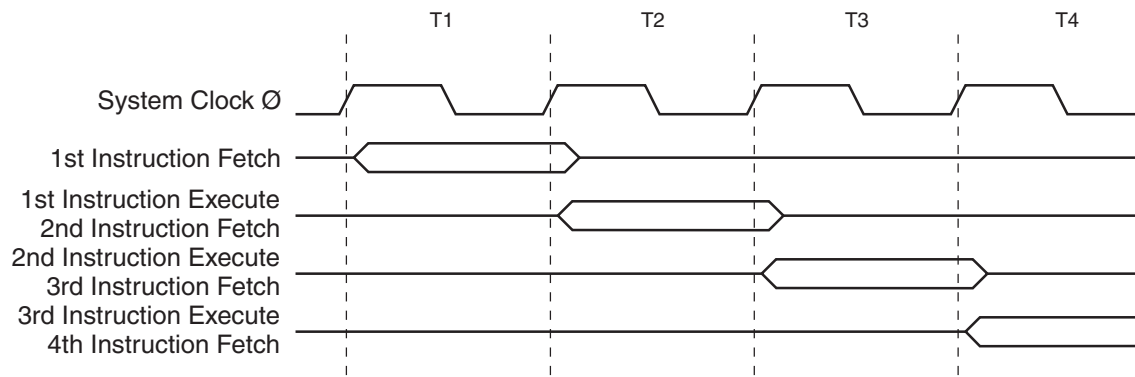
Figure 13. The Parallel Instruction Fetches and Instruction Executions
