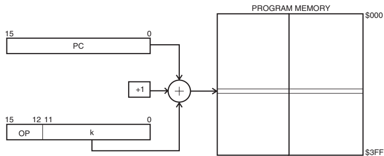
Figure 11. Relative Program Memory Addressing
