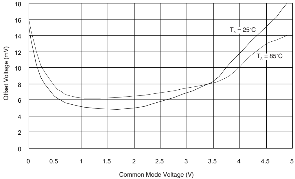
Figure 43. Analog Comparator Offset Voltage vs. Common Mode Voltage ( V_{CC}=2.7V )
