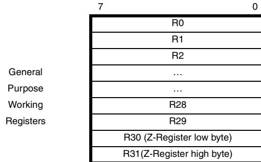
Figure 6. AVR CPU General Purpose Working Registers
