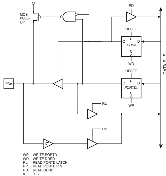
Figure 35. Port D Schematic Diagram (Pins PD7 - PD0)
