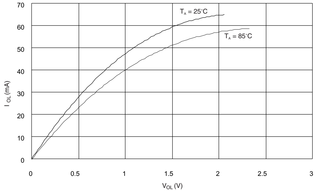
Figure 49. PA2 I/O Pin Sink Current vs. Output Voltage ( High current pin PA2; T_A=25^\circ C )
