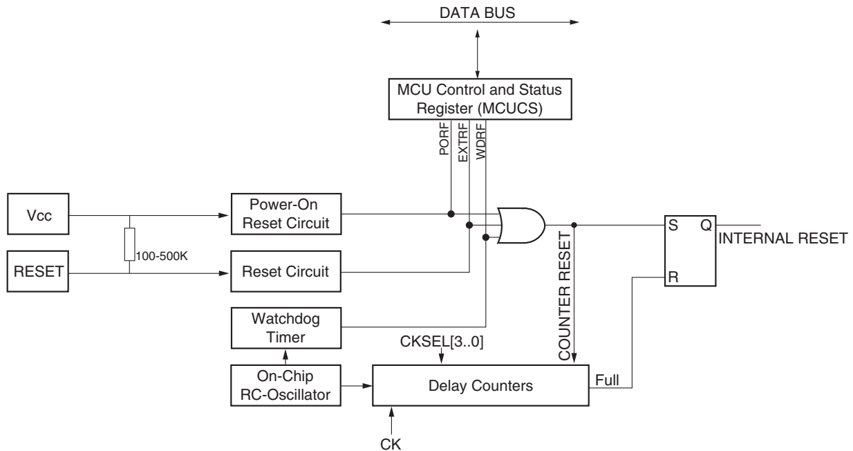
Figure 15. Reset Logic
