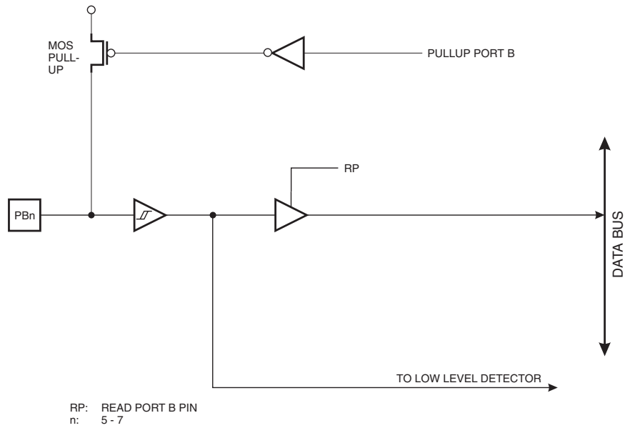
Figure 34. PORT B Schematic Diagram (Pins PB7 - PB5)
