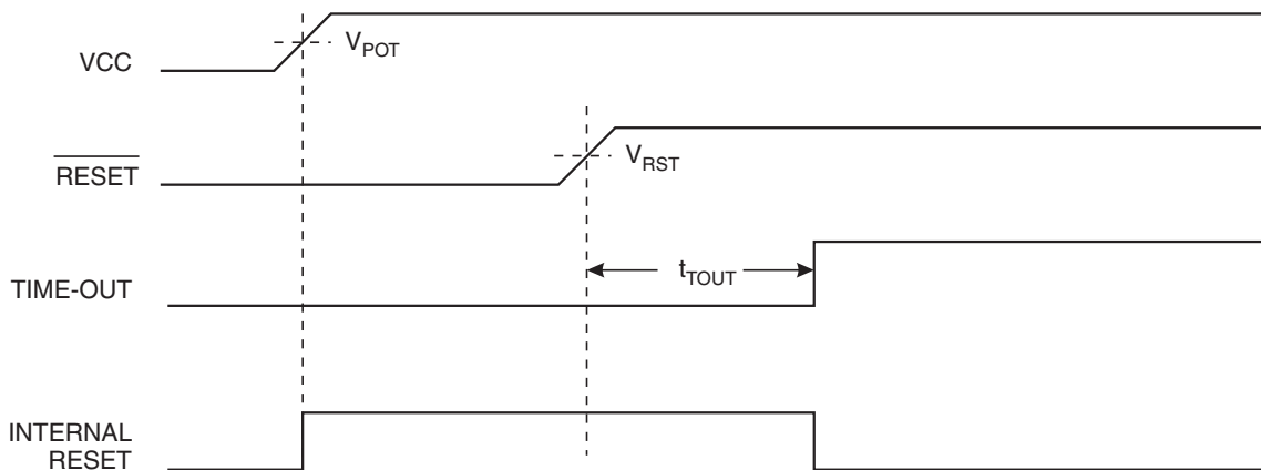
Figure 17. MCU Start-up, \overline{\text{RESET}} Controlled Externally
