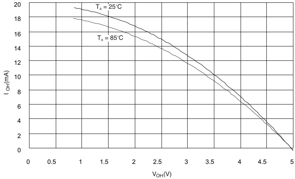
Figure 51. I/O Pin Sink Current vs. Output Voltage. All pins except PA2 ( V_{CC}= 2.7V ).
