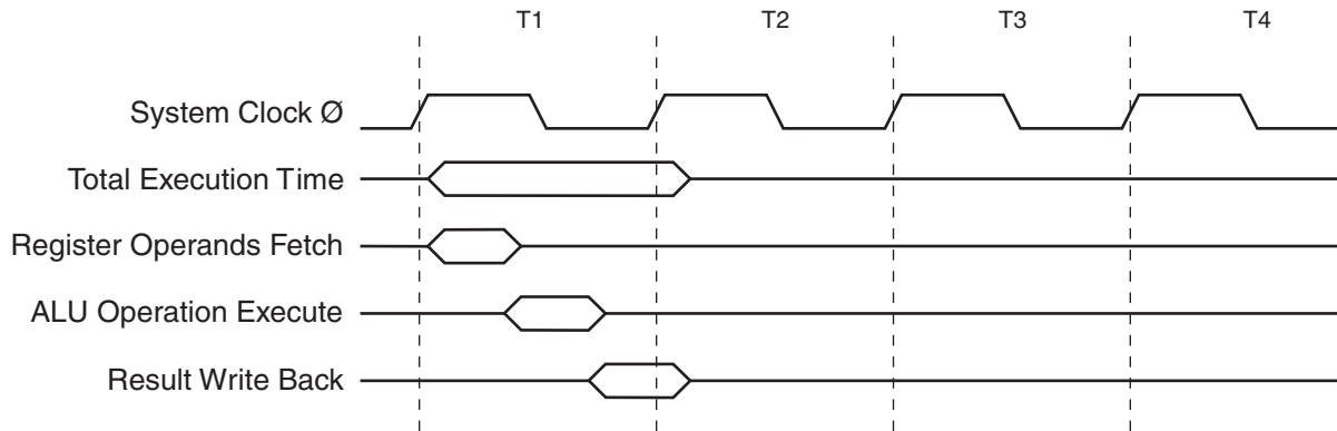
Figure 14. Single Cycle ALU Operation
