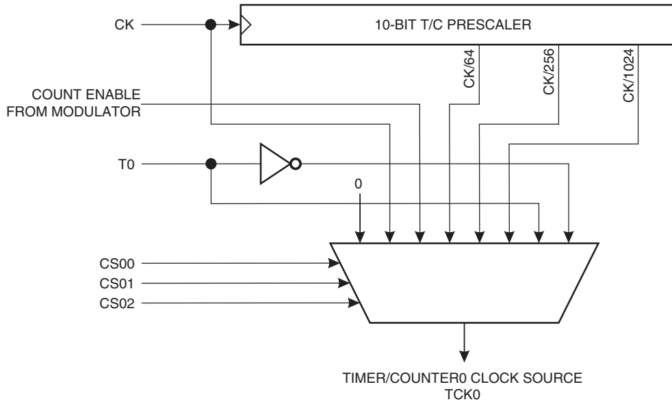
Figure 20. Timer/Counter0 Prescaler
