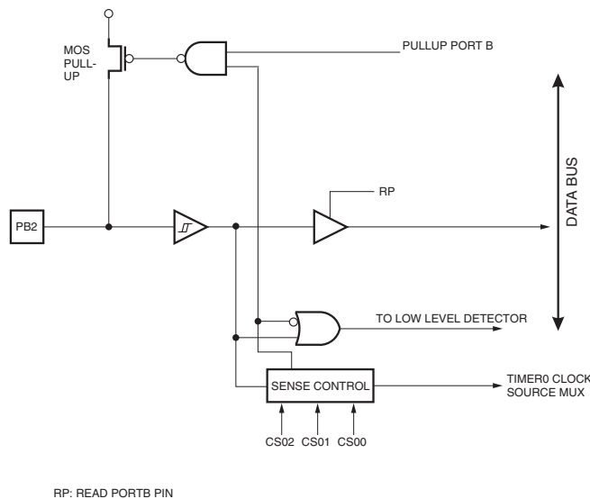
Figure 32. Port B Schematic Diagram (pin PB2)
