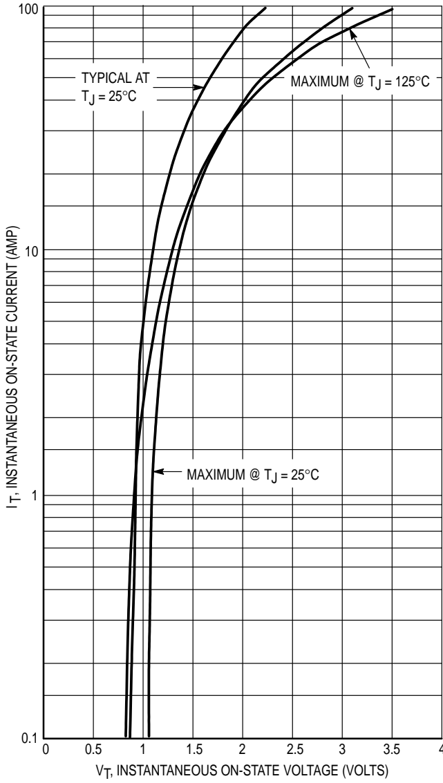
Figure 3. On-State Characteristics
