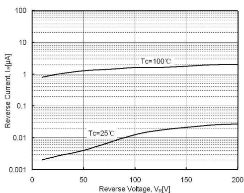
Fig. 2. Typical Characteristics: V_R vs. I_R
