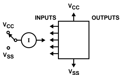
NOTE: Measure inputs sequentially, to both V CC and V SS connect all unused inputs to either V CC or V SS . FIGURE 15. INPUT CURRENT TEST CIRCUIT
