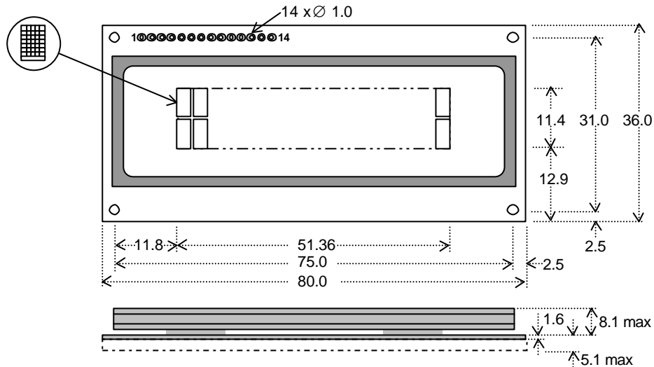
Dimensions in mm & subject to tolerances Mounting holes 2.5mm dia.
