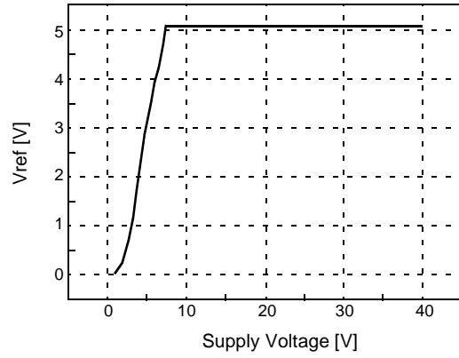
Reference Voltage
