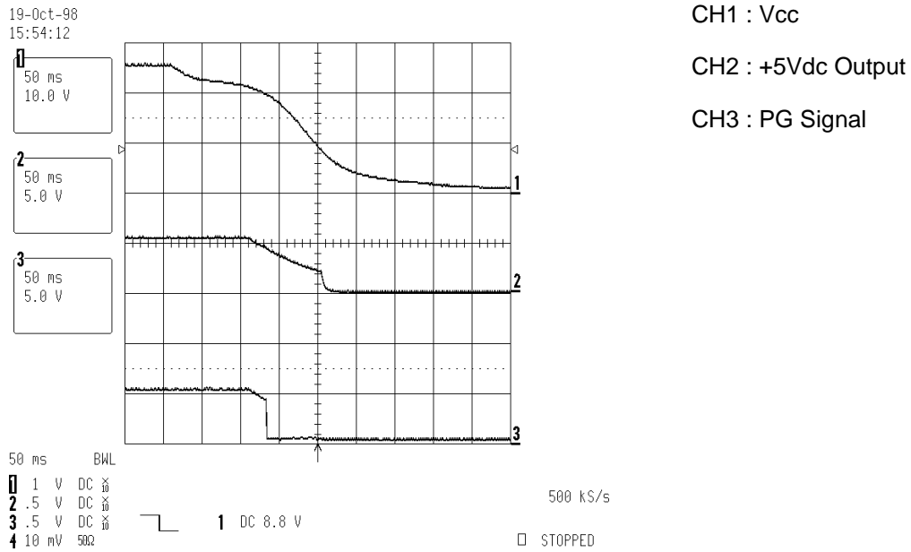
Figure 7. Vcc, +5Vdc Output vs. PG Signal (High)
