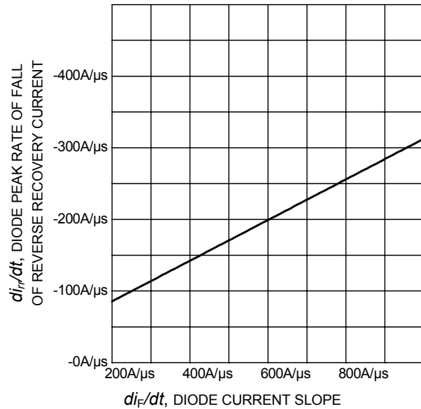
di_{rr}/dt , DIODE PEAK RATE OF FALL OF REVERSE RECOVERY CURRENT di_F/dt , DIODE CURRENT SLOPE Figure 24. Typical diode peak rate of fall of reverse recovery current as a function of diode current slope ( V_R=400V , T_J=150^\circ C , Dynamic test circuit in Figure E)
