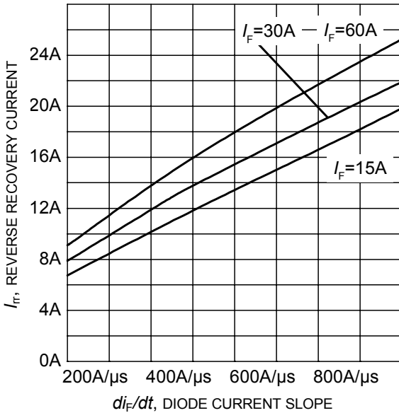
I_{rr} , REVERSE RECOVERY CURRENT di_F/dt , DIODE CURRENT SLOPE Figure 23. Typical reverse recovery current as a function of diode current slope ( V_R=400V , T_J=150^\circ C , Dynamic test circuit in Figure E)
