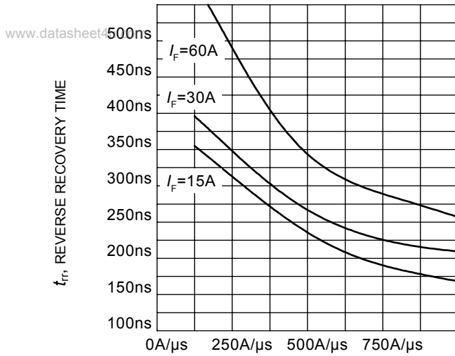
di_F/dt , DIODE CURRENT SLOPE Figure 21. Typical reverse recovery time as a function of diode current slope ( V_R=400V , T_J=150^\circ C , Dynamic test circuit in Figure E)
