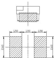
推荐焊盘 Recommended Soldering Pad
